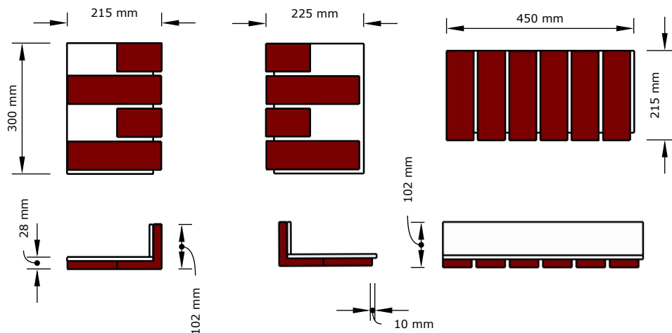
Standard cladding panel
